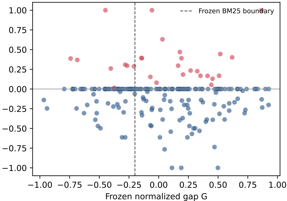
POST-HOC: confidence gap vs actual advantage
