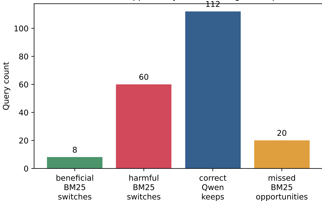
POST-HOC: BM25 opportunity and switching decomposition
