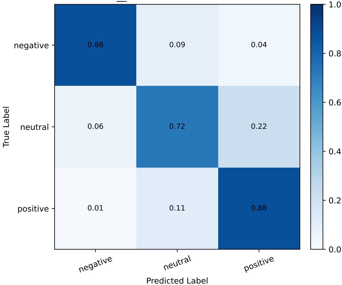
Normalized Confusion Matrix hfl_chinese-roberta-wwm-ext
