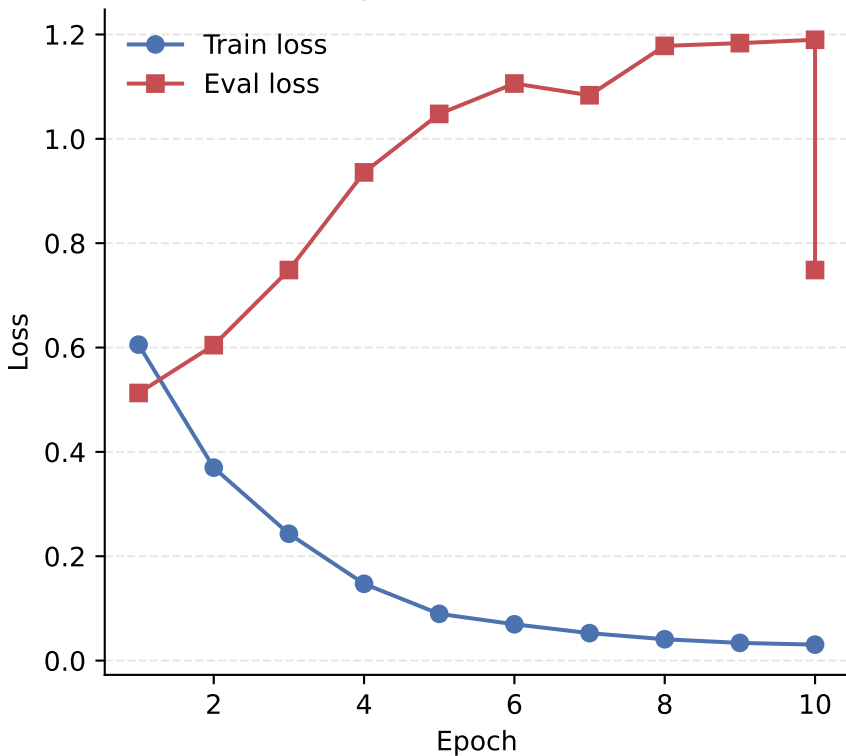
Training and Evaluation Loss
