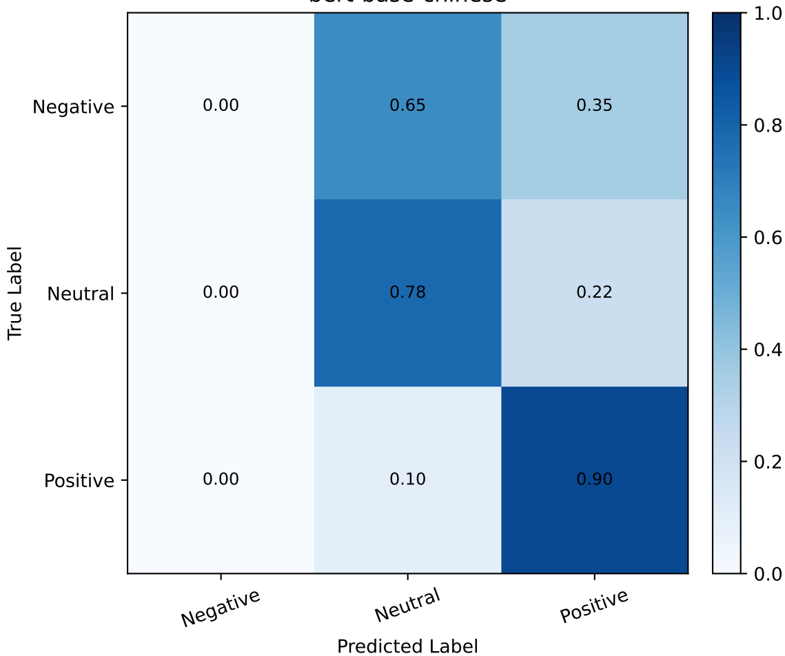
Normalized Confusion Matrix bert-base-chinese
