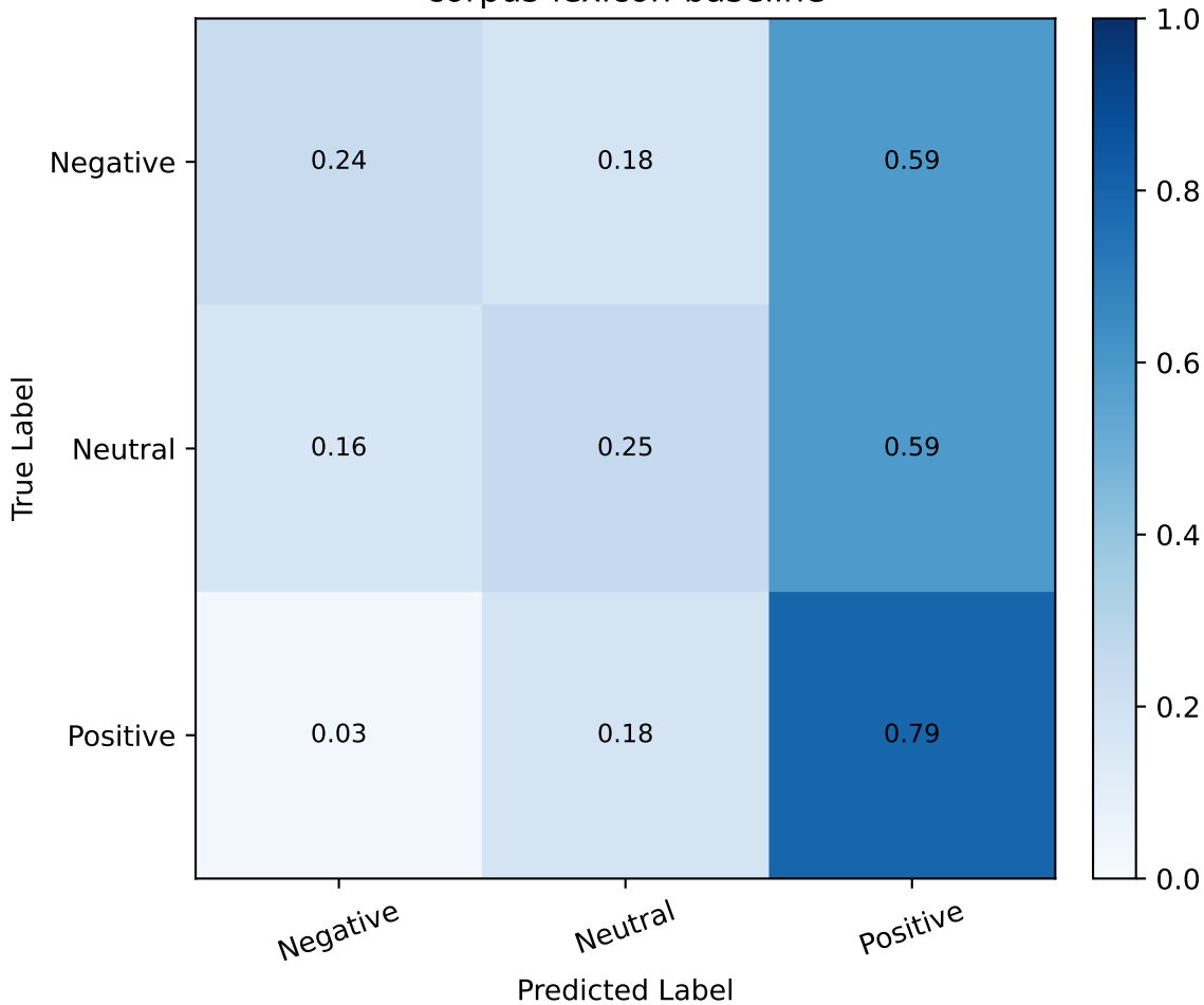
Normalized Confusion Matrix corpus-lexicon-baseline
