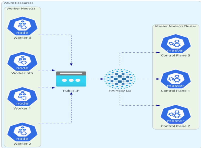
Figure: HLD Local ETCD
