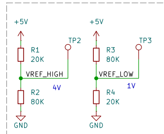
Comparator Voltage Reference Window
