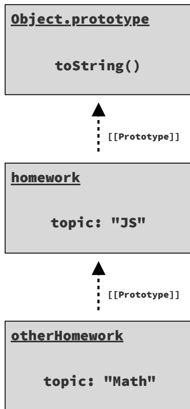
Fig. 5: Shadowed property ‘topic’
