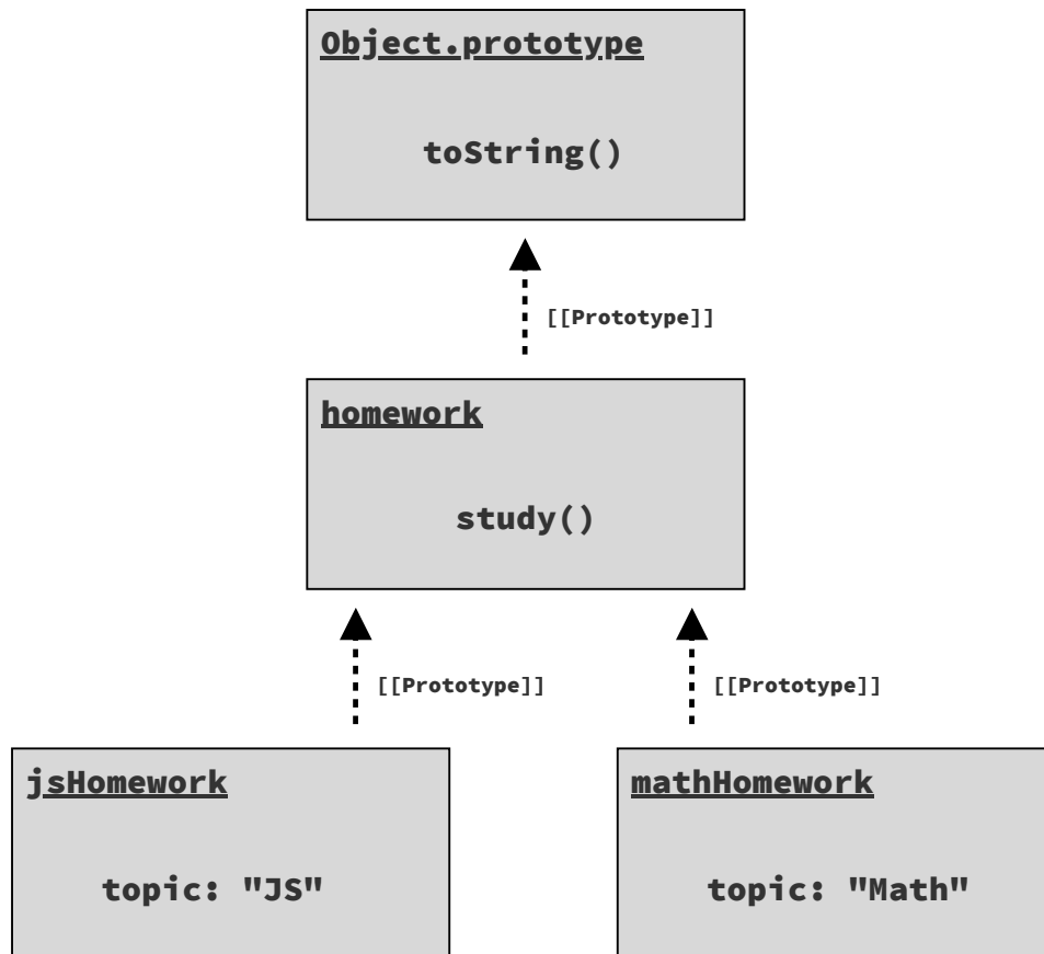
Fig. 6: Two objects linked to a common parent
