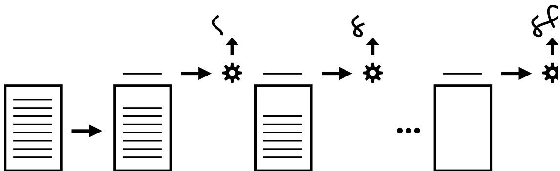
Fig. 1: Interpreted/Scripted Execution
