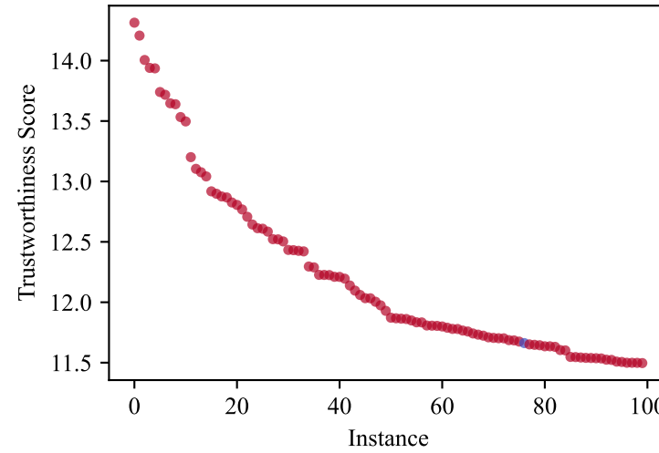
CAGED (0 to 100)
