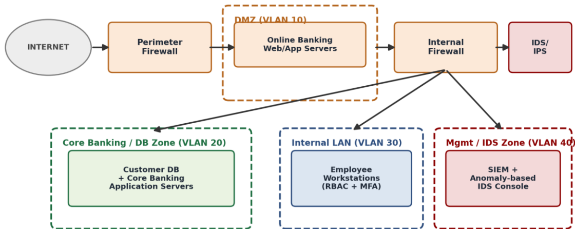
Figure 3: Segmented Financial Institution Network with Two-Tier Firewall and Hybrid IDS
