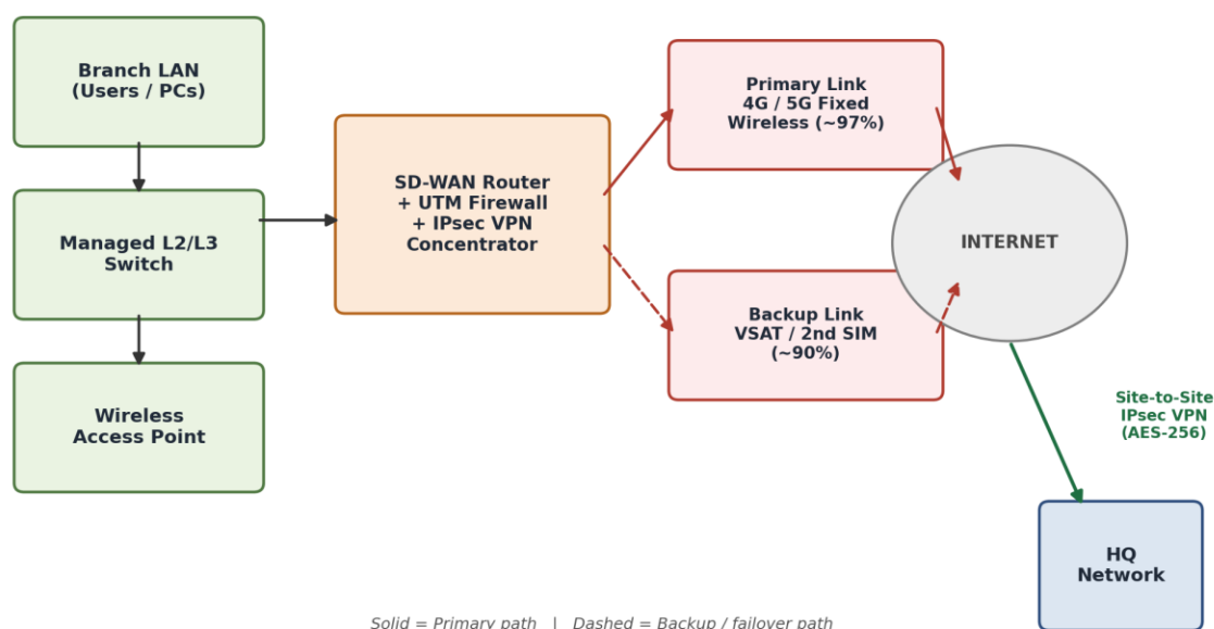
Figure 1: Recommended branch office network architecture — dual-WAN (primary 4G/5G + backup VSAT/SIM) behind an SD-WAN router with UTM firewall, connected to HQ via a site-to-site IPsec VPN tunnel.
