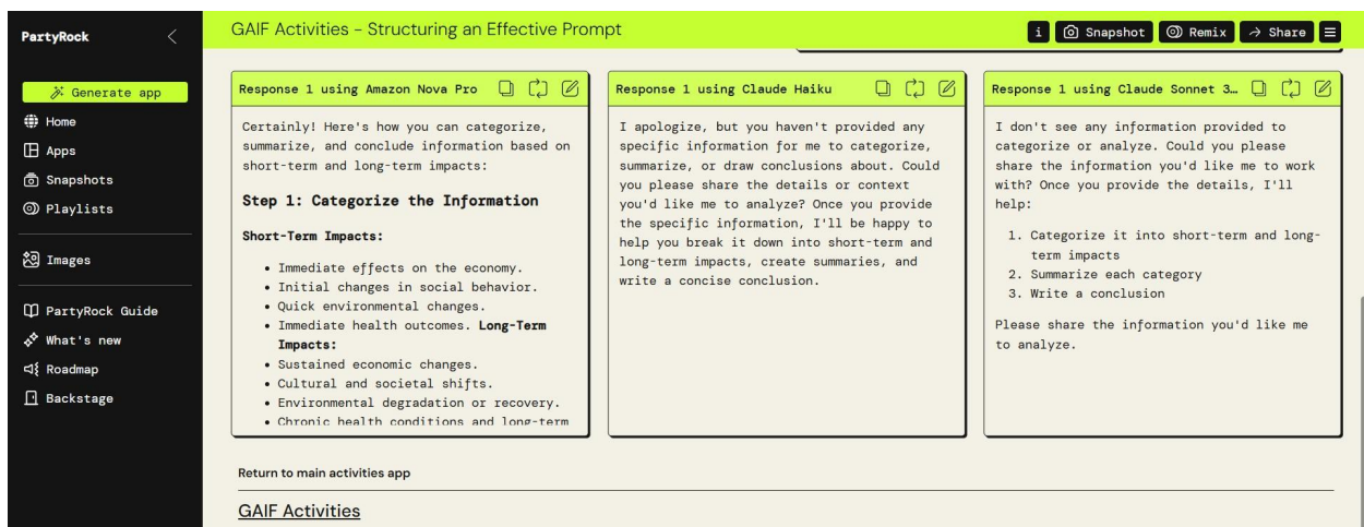
Figure 4:Part1ex2- output
