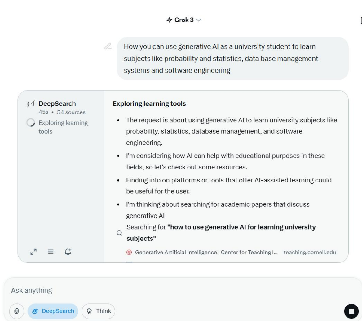
Figure 12: Using DeepSearch
