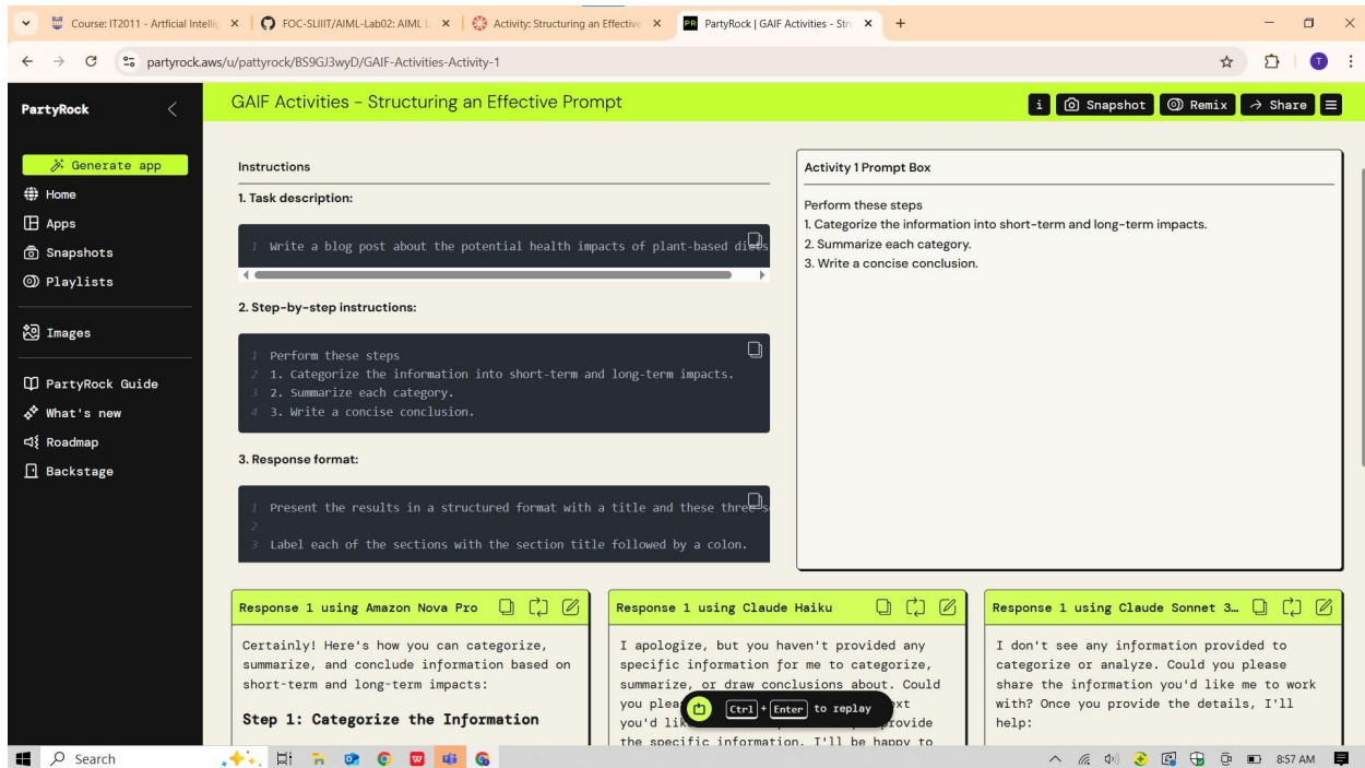
Figure 3:Part1ex2- prompt
