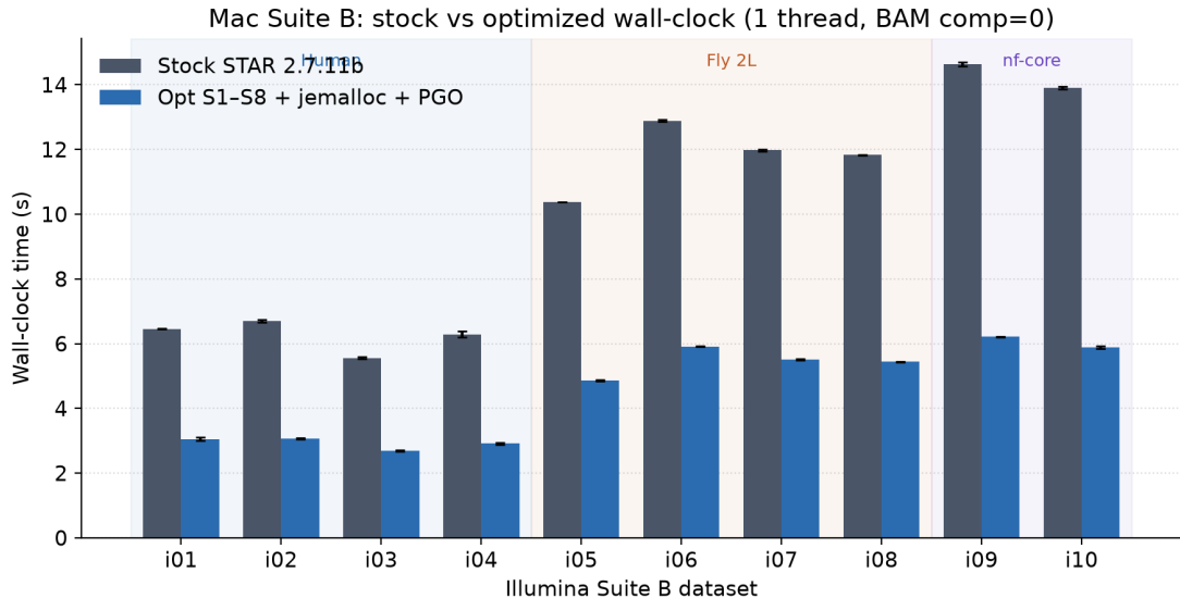
Figure 3: End-to-end wall-clock (mean ± std) for stock and ACTS on Suite B. Shaded bands mark human, fly 2L, and nf-core index families.
