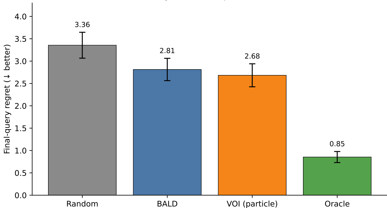
VOI ablation — final regret (n=150 paired user-runs, mean \pm SE)
