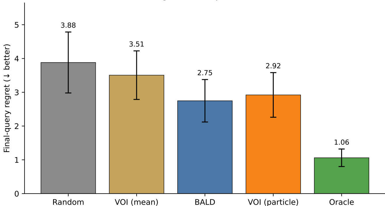
VOI ablation — final regret (n=24 paired user-runs, mean \pm SE)
