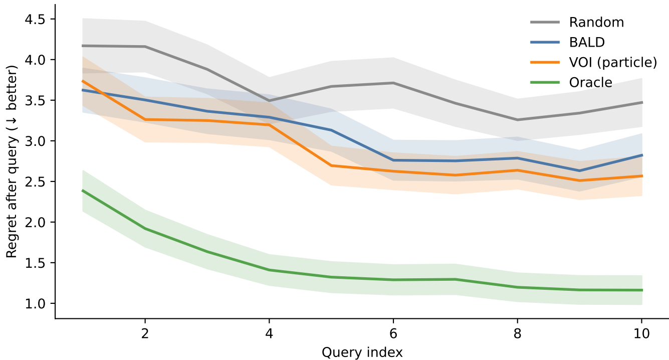
Regret curves — mean \pm SE
