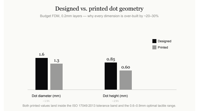
Fig. 5. Designed versus printed dot geometry on budget FDM printers. Both printed values land inside the ISO 17049:2013 tolerance band and the 0.6 to 0.9 millimeter range identified as optimal in blind-reader surveys, confirming that the 20 to 30 percent over-design correction is calibrated rather than arbitrary.
