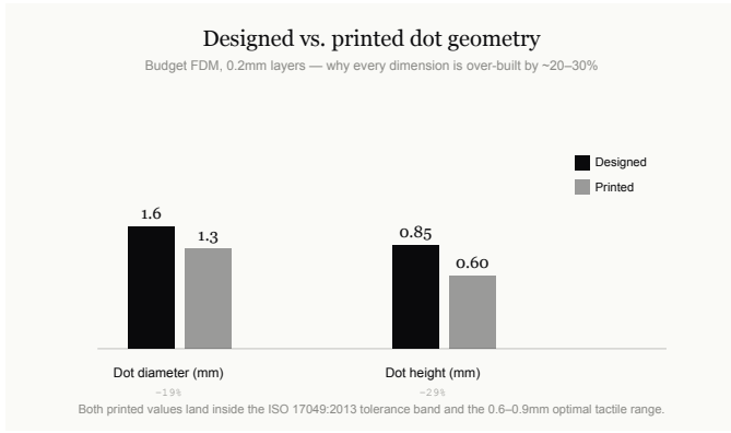
Fig. 4. Designed versus printed dot geometry on budget FDM printers. Both printed values land inside the ISO 17049:2013 tolerance band and the 0.6 to 0.9 millimeter range identified as optimal in blind-reader surveys, confirming that the 20 to 30 percent over-design correction is calibrated rather than arbitrary.
