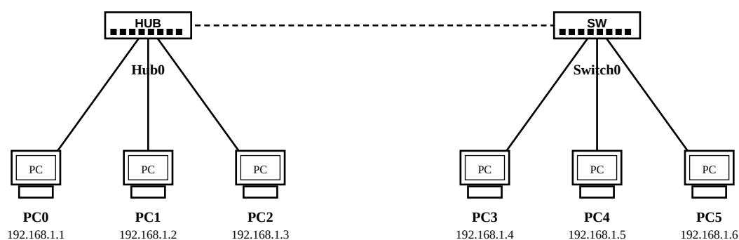
Fig 3: Network using both HUB and SWITCH (6 hosts)
