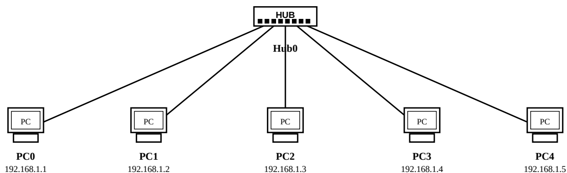
Fig 1: Network using only a HUB (5 hosts)
