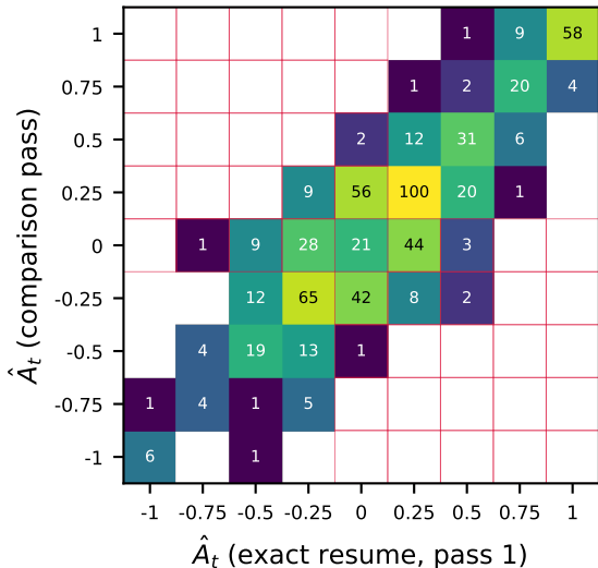
re-feed vs exact resume sign flips: 205/622 = 33.0%
