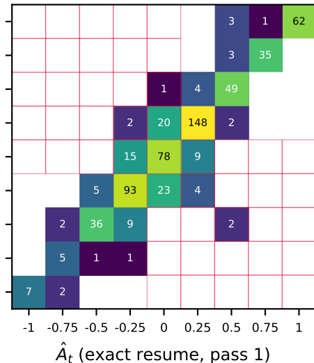
exact replica vs exact resume (floor) sign flips: 76/622 = 12.2%
