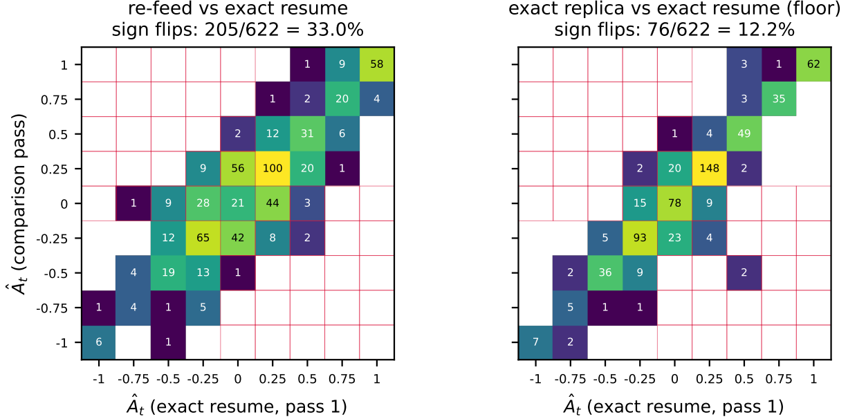
Figure 1: Joint distribution of \hat{A}_t under exact resume (x-axis) and the comparison pass (y-axis), pooled main configuration, common eligible set ( n = 622 ). Cells outlined in red disagree in sign with exact pass 1. Left: the re-feed pass scatters 33.0% of estimates into sign-disagreeing cells. Right: an identical exact replica pass, the noise floor, scatters 12.2%.
