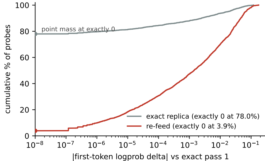
Figure 3: Cumulative distribution of the absolute first-token logprob delta against exact pass 1, over 3,127 greedy probes pooled across the full runs. Resuming the decode-time state is bit-exact at 78.0% of probes; re-feeding is bit-exact at 3.9% and exhibits a tail an order of magnitude heavier.
