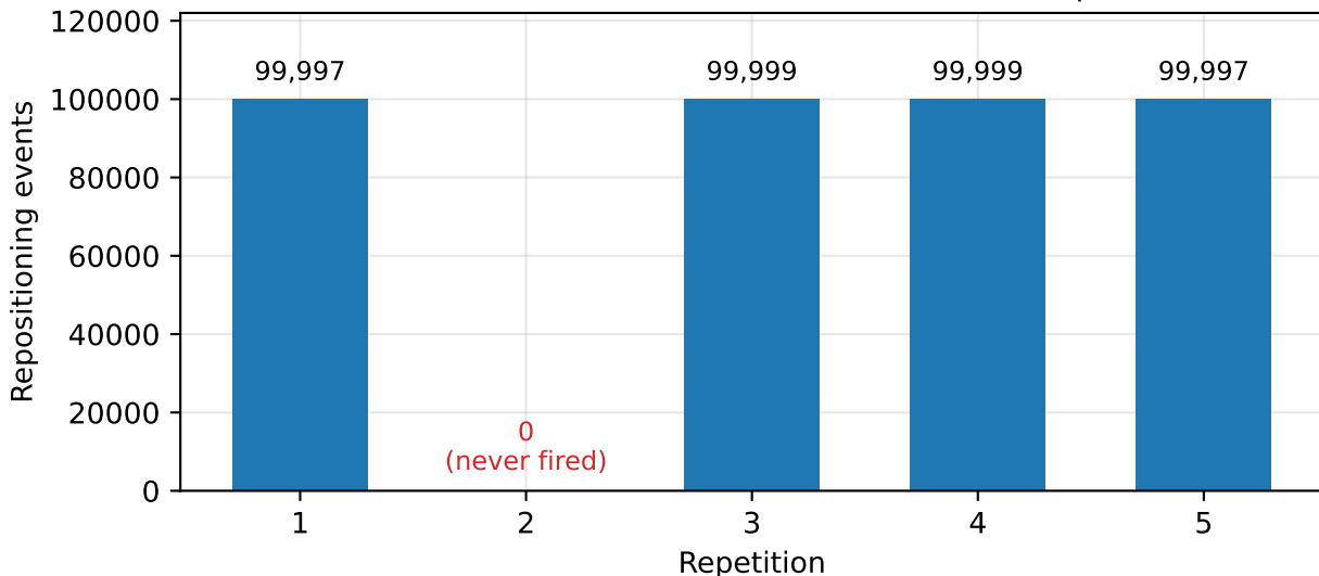
(a) Threshold-Naive: bimodal outcome (N = 100,000 packets)
