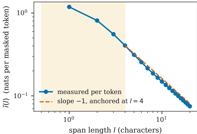
(b) decay over the fit range: -1.03 vs -1
