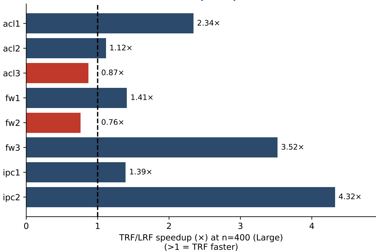
(b) Per-ruleset speedup at n=400
