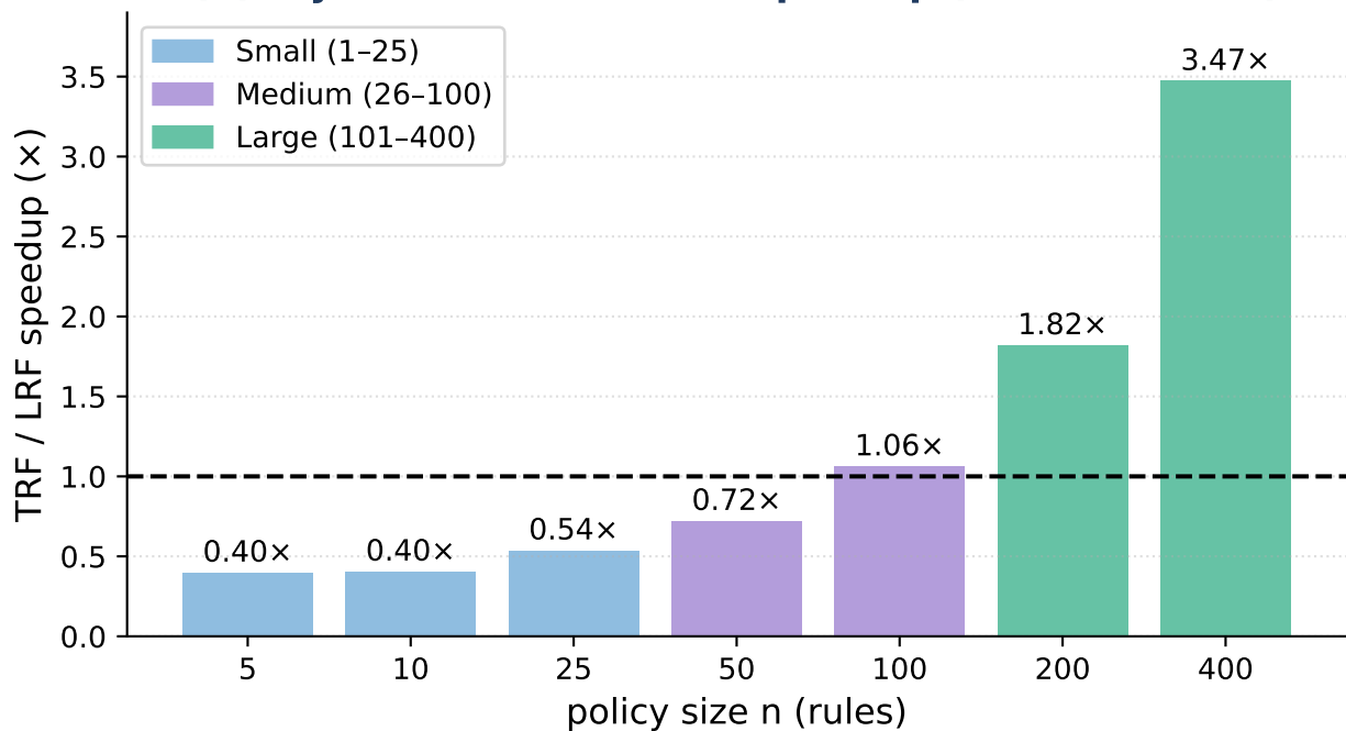
(b) Python-level TRF/LRF speedup (same runtime)
