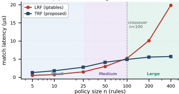
(a) Match latency: TRF vs LRF
