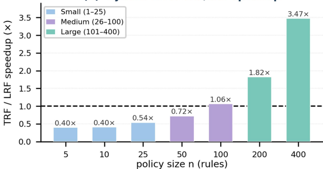
(b) Python-level TRF/LRF speedup
