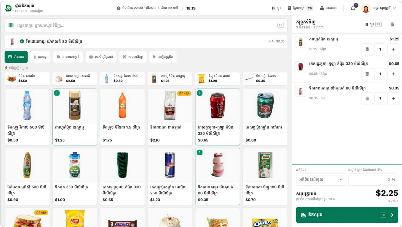
Figure 2. The terminal: grid, cart and pay button. Shortcuts are printed on the buttons.
