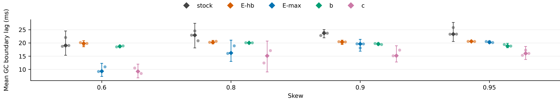
GC boundary and live versions · 計器入り build の診断値 48 threads, 1M tuples, 50% reads, wait 10 ms, GC 10 \mu s
