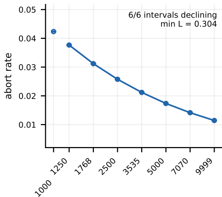
fixed static backoff (us)
