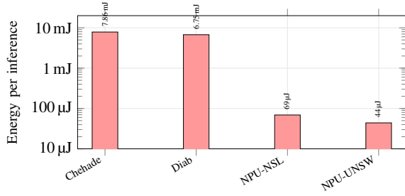
Fig. 2. Energy per inference (log scale). Our NPU path achieves over two orders of magnitude reduction versus CPU-only MCU baselines. NPU = ReLU INT8 on Neural-ART (estimated from AN5946). Chehadé [1]: STM32F7; Diab [2]: RPi 3B+.
