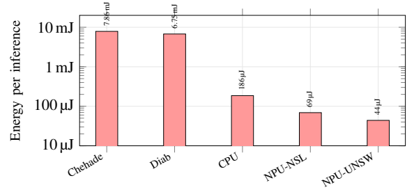
Fig. 2. Energy per inference comparison (log scale). NPU deployment achieves over 100 \times reduction versus CPU-only MCU baselines. CPU = ReLU FP32 on Cortex-M55; NPU = ReLU INT8 on Neural-ART. Chehade [1]; STM32F7; Diab [2]; RPi 3B+.
