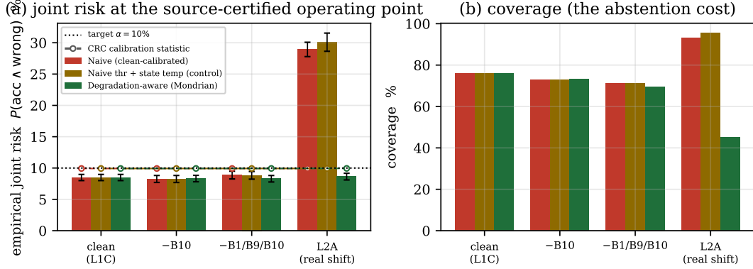
Figure 1: Naive conformal exceeds its nominal 10% target under the L1C → L2A shift while Mondrian restores control (proposed model, 100 runs, two-way cluster-robust SE). (a) empirical joint risk at the certified operating point, per state, with error bars the small-cluster t_9 95% CI; (b) coverage, the abstention cost of the remedy. The dashed lines are the reused source-domain CRC calibration selection statistic (never re-validated on target outcomes), which stays \leq \alpha throughout even as the naive L2A risk soars to 27.8%—the sense in which the failure is silent.
