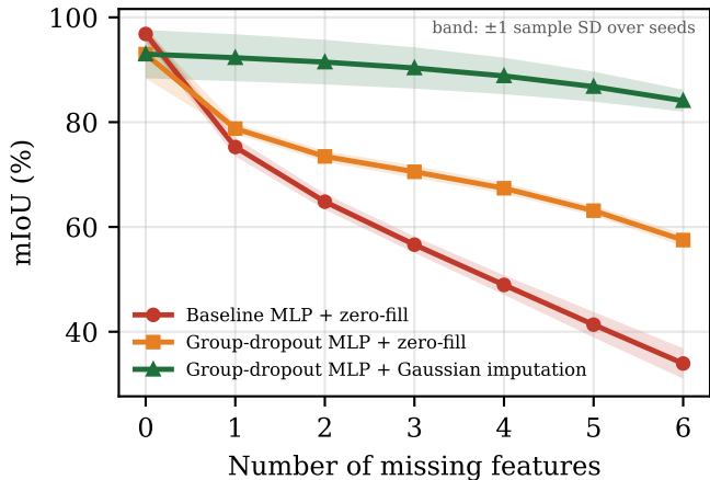
Missing-feature robustness (synthetic, 5 seeds)
