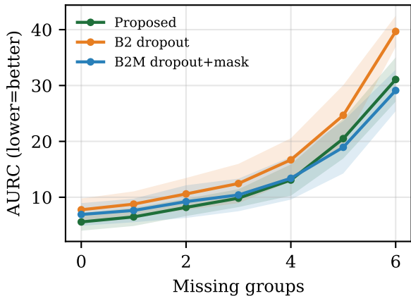
Selective risk (AURC)
