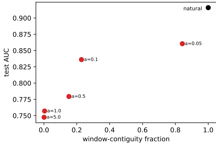
(b) contiguity vs AUC: Spearman \rho = 1.00
