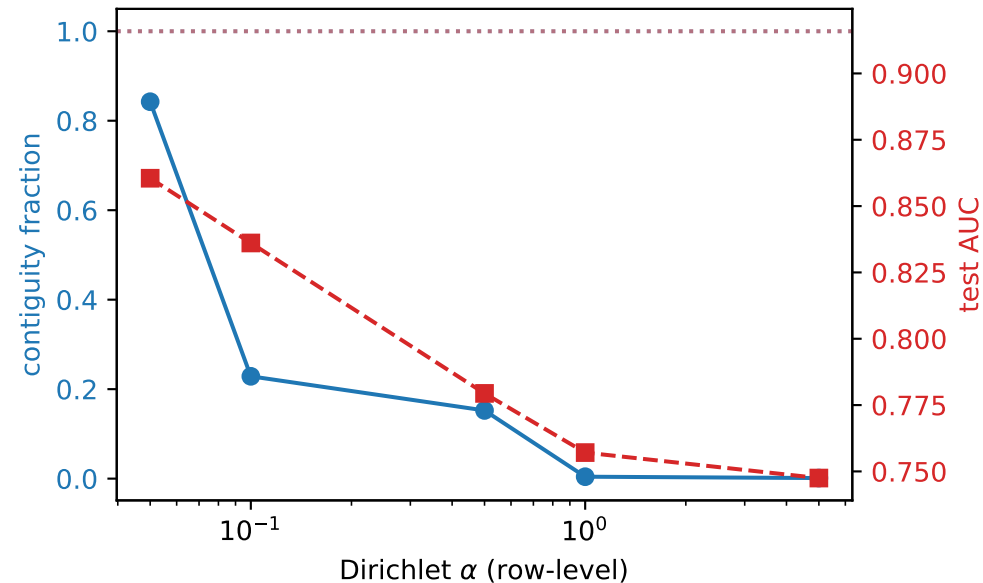
(a) both fall monotonically with \alpha
