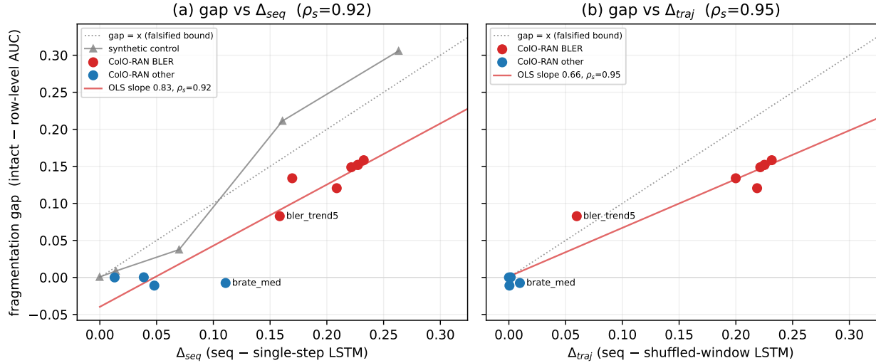
Fig. 1. The fragmentation AUC gap (intact – row-level) is a monotone function of the sequence-essentiality diagnostic. (a) vs. \Delta_{seq} (seq – single-step LSTM), with the synthetic controlled backbone and the gap = x line (the falsified bound ). (b) vs. the order-isolating \Delta_{traj} (seq – shuffled-window LSTM): tighter ( \rho_s=0.95 ) and pulls the persistent brate_med deviator onto the origin. Order-free targets (CQI/MCS/buffer/throughput) cluster at gap \approx 0 ; BLER targets rise with the diagnostic. Slopes < 1 in (b) reflect \Delta_{traj} \geq \text{gap} (it over-predicts; Sec. V).
