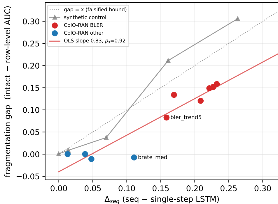
(a) gap vs \Delta_{seq} ( \rho_s=0.92 )
