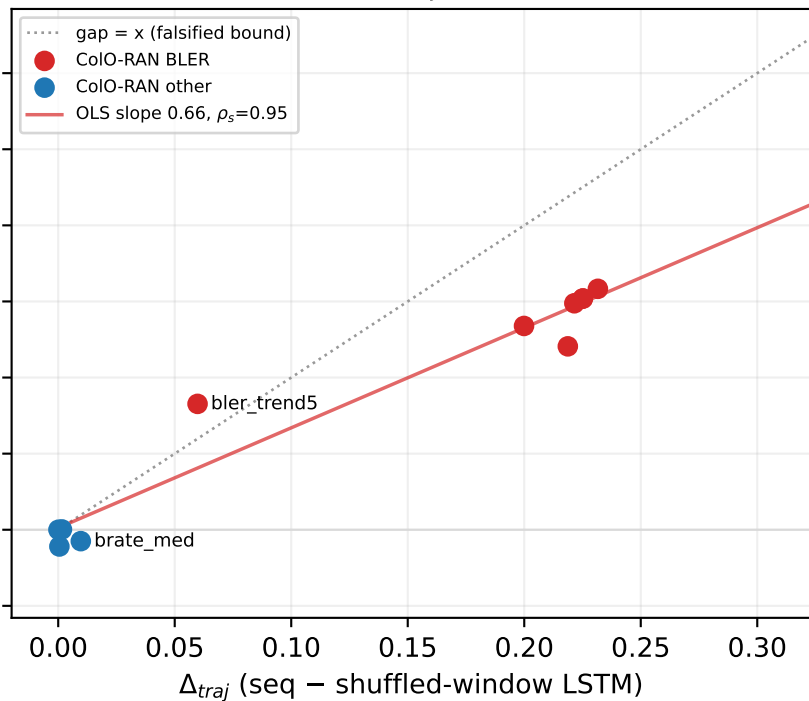
(b) gap vs \Delta_{traj} ( \rho_s=0.95 )
