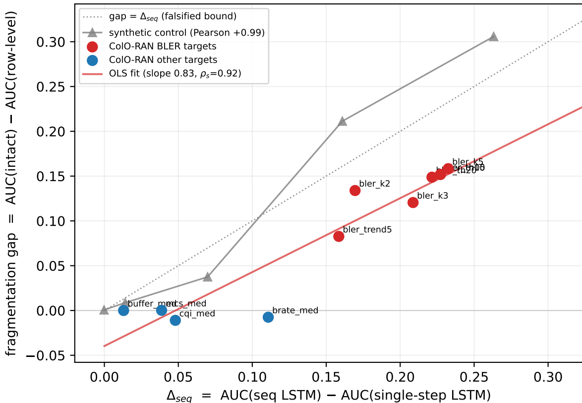
Fragmentation AUC gap tracks sequence-essentiality ( \Delta_{seq} )
