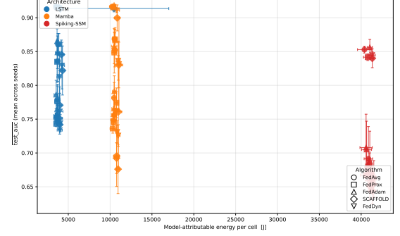
Phase 5 — Pareto: test AUC vs model-attributable energy (90 groups, 900 cells; Mamba uses pure-PyTorch sequential scan, not Triton kernel)
