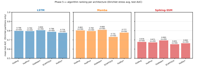
Fig. 1. Per-architecture algorithm ranking (mean test AUC, averaged over Dirichlet partitions \alpha_{\text{dir}} \in \{0.05, 0.10, 0.50, 1.00, 5.00\} and 10 seeds; n = 50 per bar; switched from best-val to test AUC per reviewer Minor#2). Three panels: LSTM / Mamba / Spiking-SSM.
