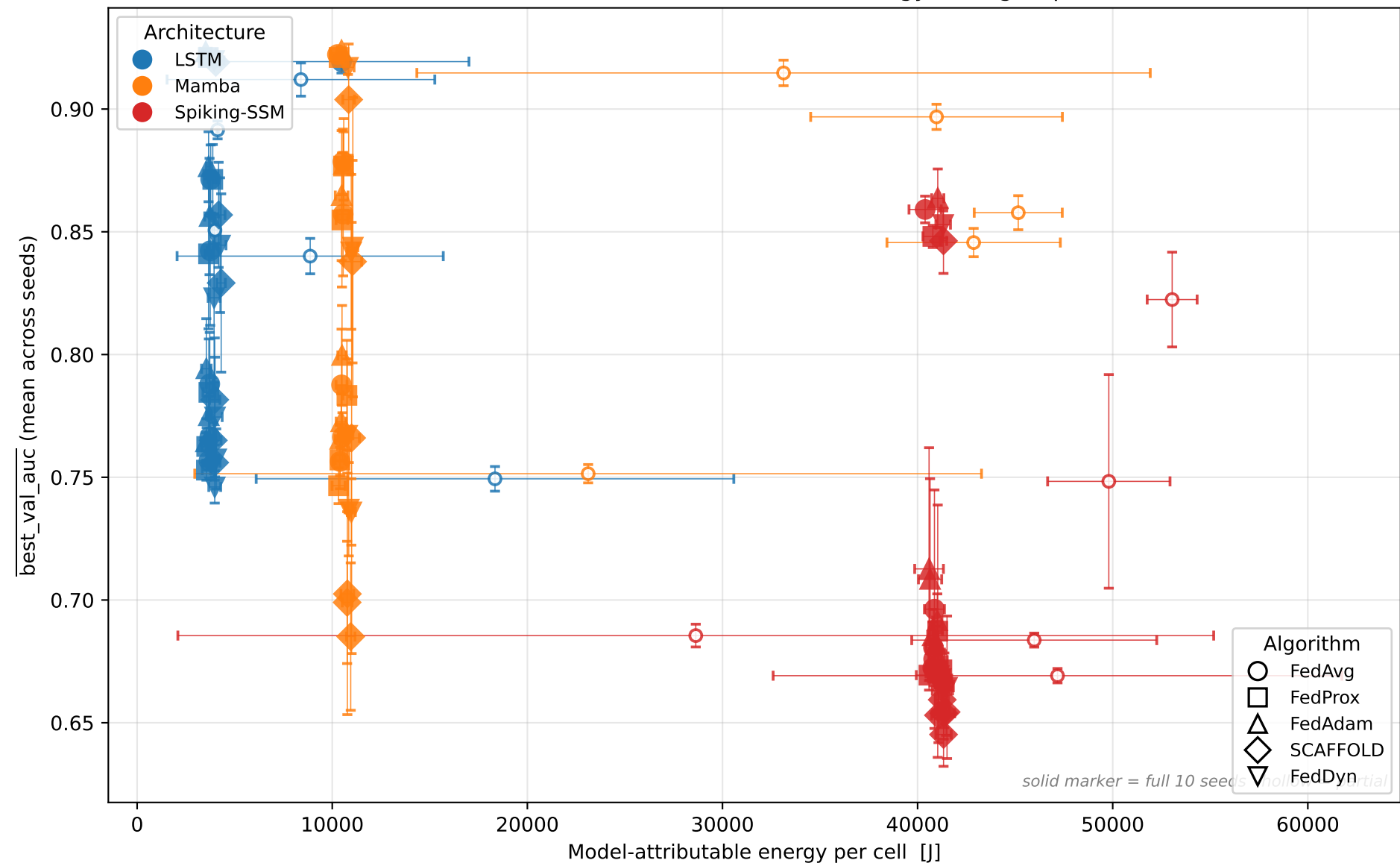
Phase 5 — Pareto: AUC vs model-attributable energy (105 groups, 975 cells)
