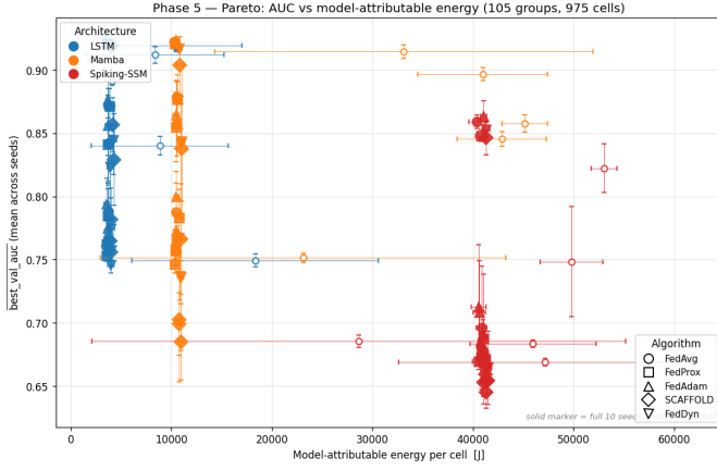
Fig. 3. Energy–AUC Pareto front on RTX 4080. Per-cell mean best-validation AUC vs per-cell NVML idle-baseline-subtracted training energy (kJ). Points coloured by architecture (LSTM blue, Mamba orange, Spiking-SSM red); marker shape encodes algorithm. Three vertical bands at 3.51–4.31 / 10.27–11.06 / 40.39–41.51 kJ/cell.
