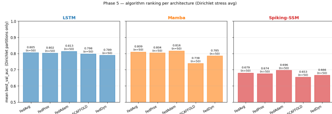
Fig. 1. Per-architecture algorithm ranking (mean best-validation AUC, averaged over Dirichlet partitions \alpha_{\text{dir}} \in \{0.05, 0.10, 0.50, 1.00, 5.00\} and 10 seeds; n = 50 per bar). Three panels: LSTM / Mamba / Spiking-SSM.
