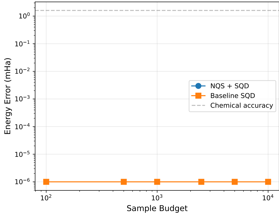
LiH: Error vs Sample Budget
