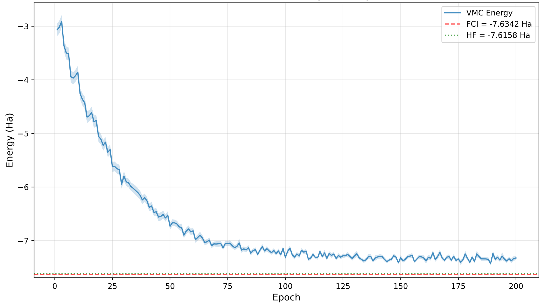
LiH (STO-3G): VMC Training Convergence
