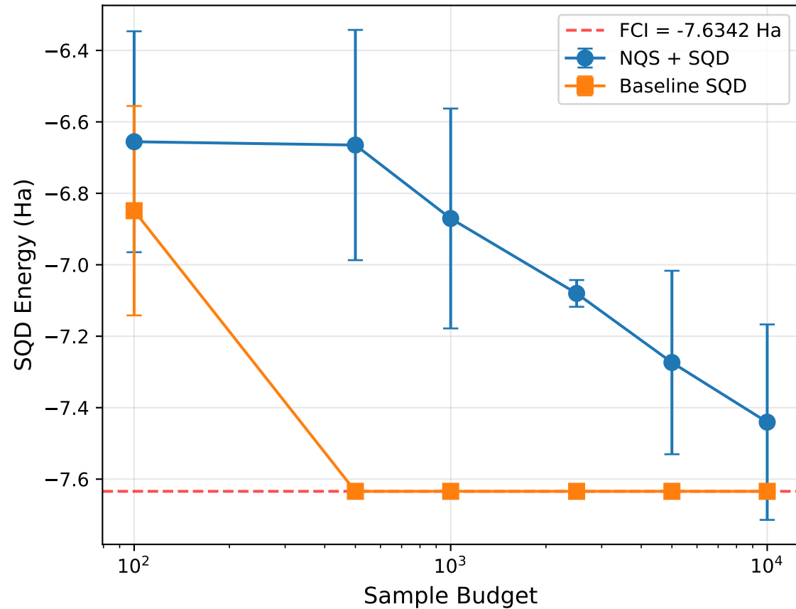
LiH: SQD Energy vs Sample Budget
