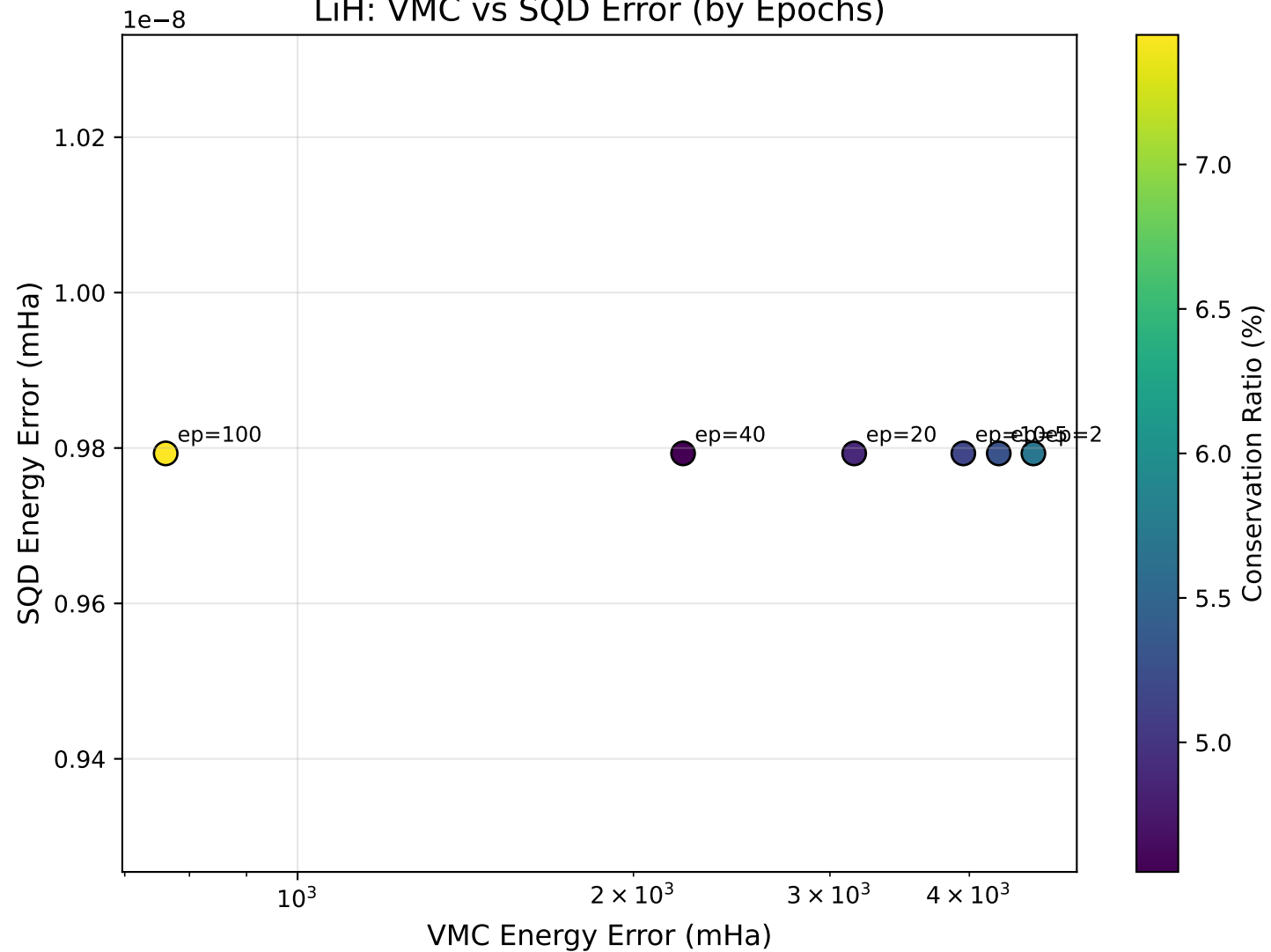
LiH: VMC vs SQD Error (by Epochs)
