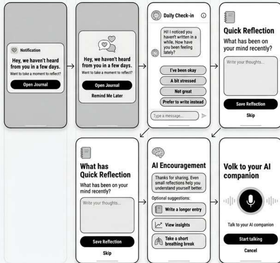
Mobile Check-in Flow (Android)
