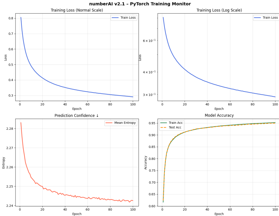
Figure 5: Version 2.1 Training Loss Progression (8 Kernels)
