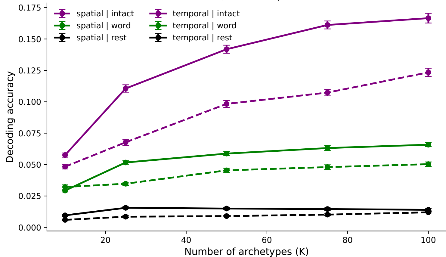
Decoding vs raw K | across
