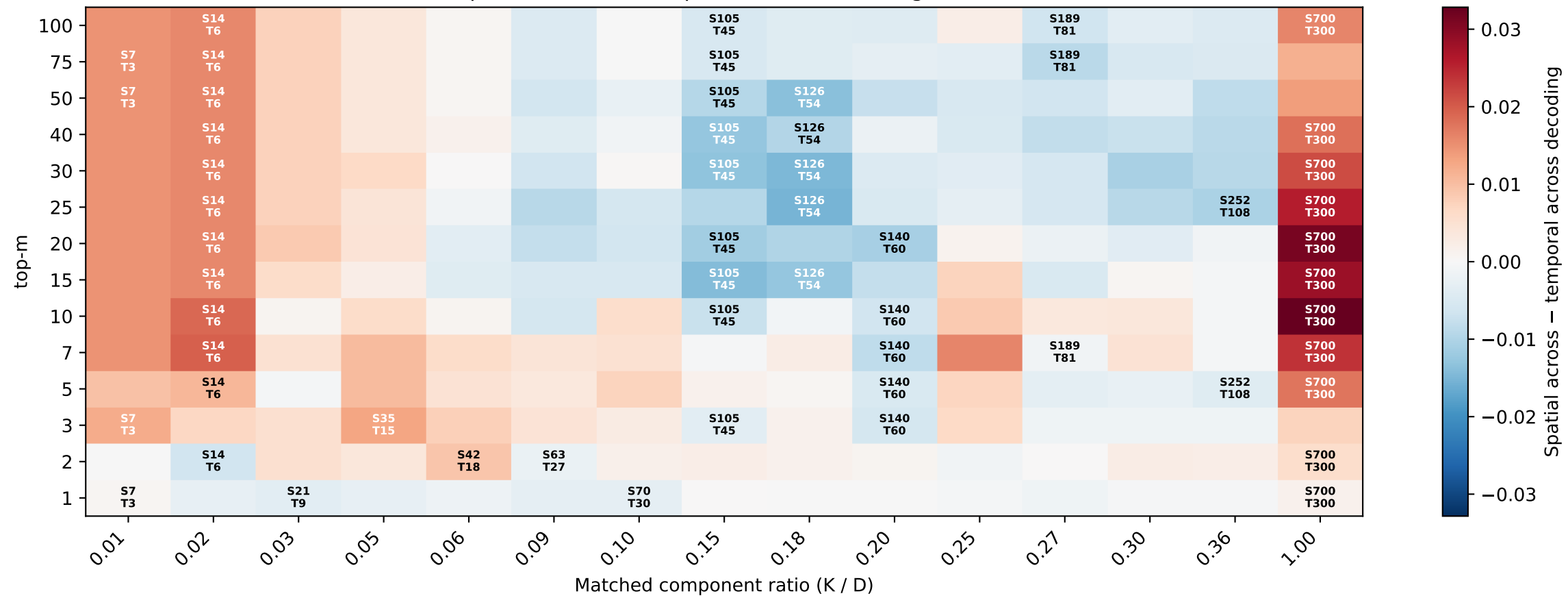
Spatial across – temporal across decoding: word
