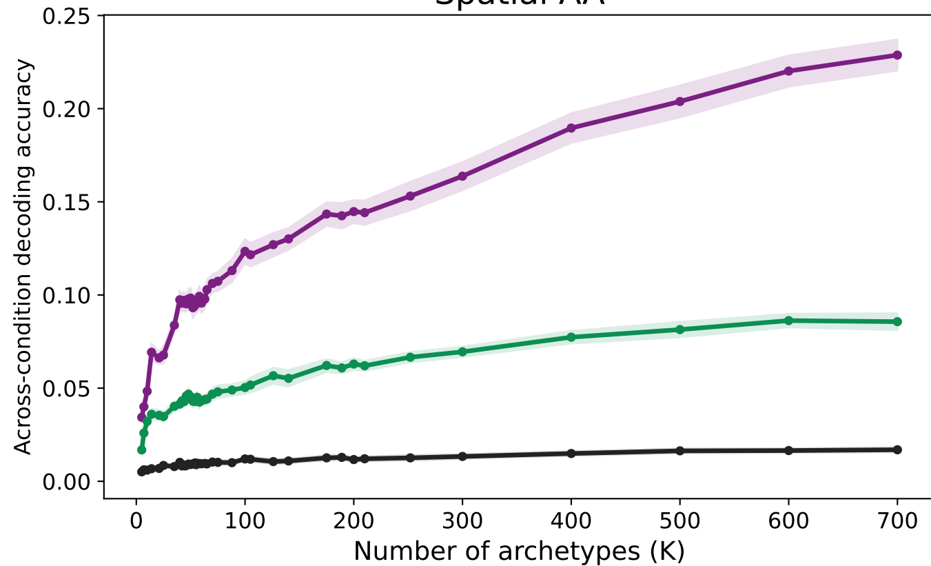
Spatial AA
