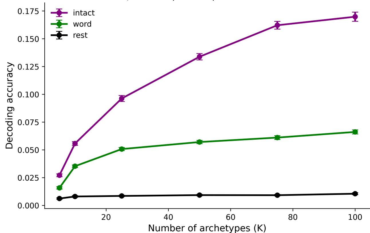
Temporal AA | within | full reconstruction
