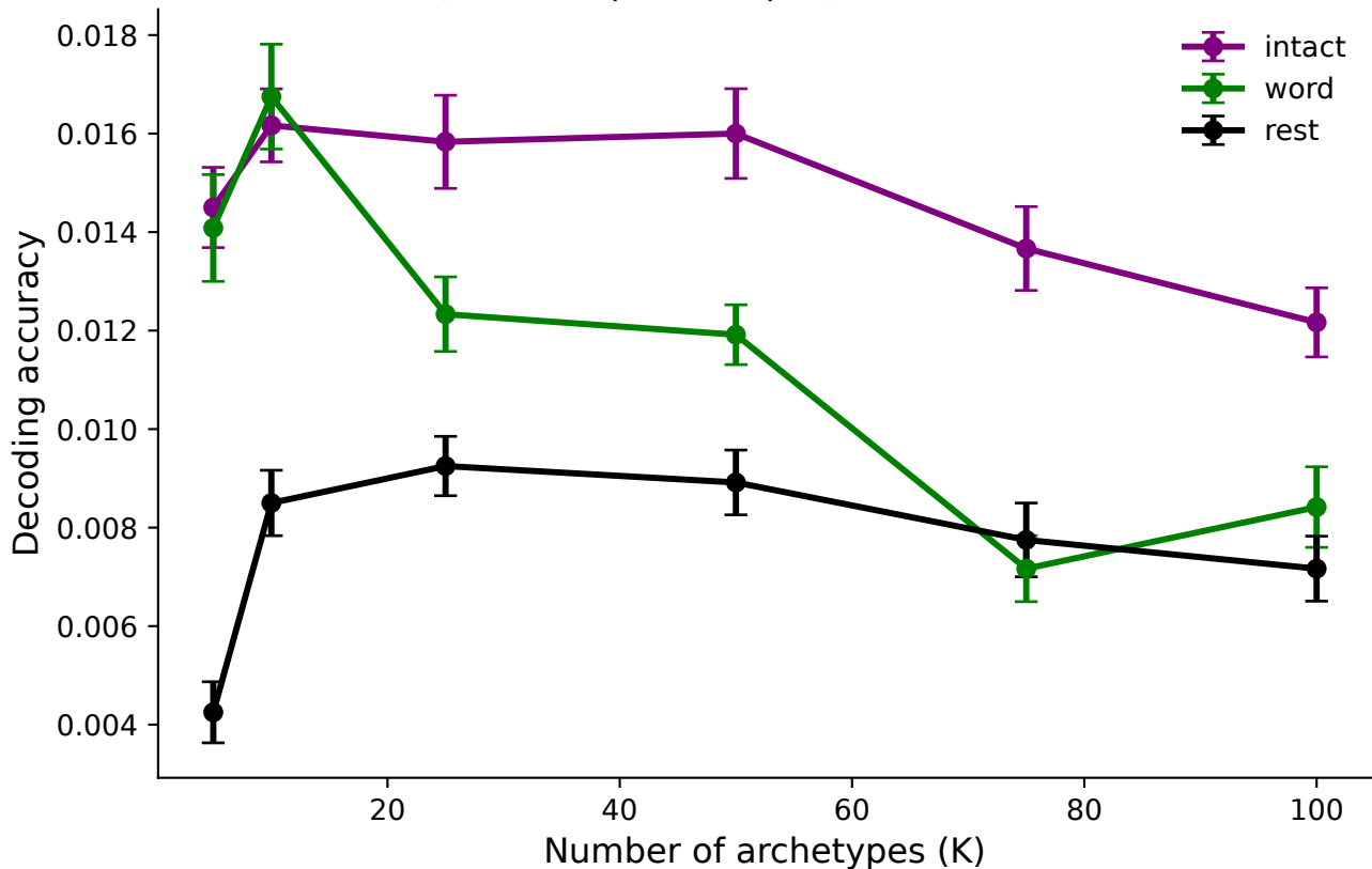
Temporal AA | across | top-2 reconstruction
